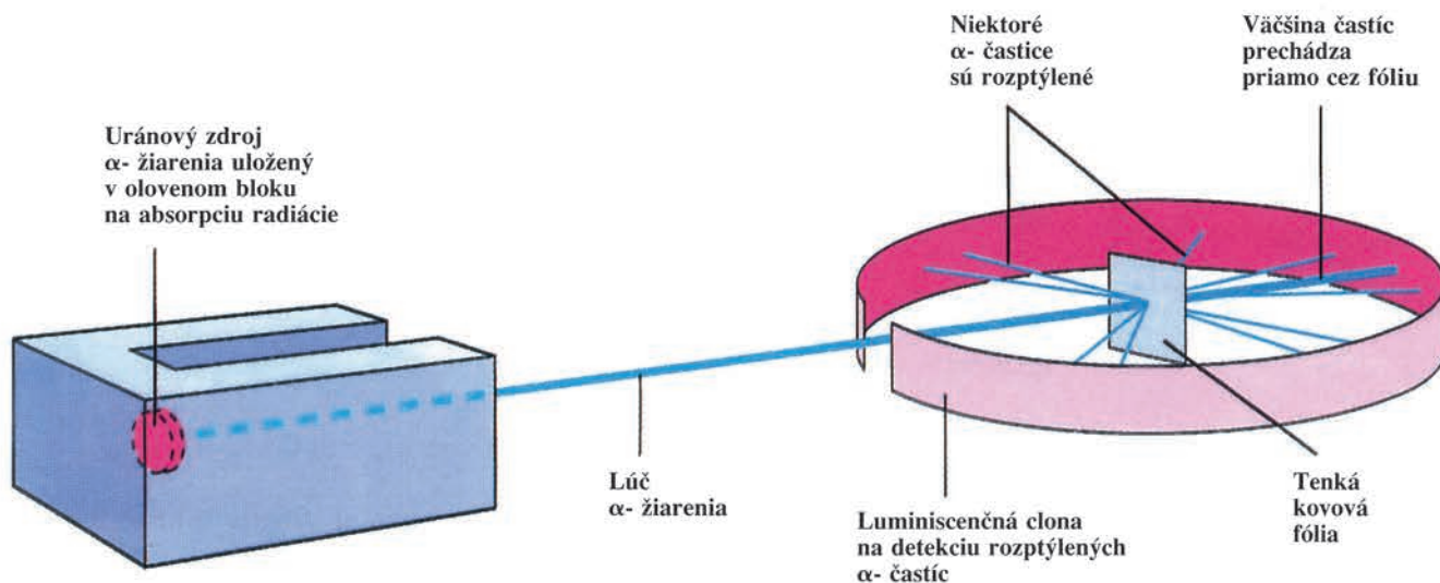
Obr. 1.1 Rutherfordov pokus
